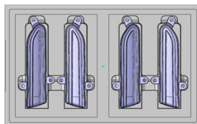
Container design with 4 cavities for left or right unit.
