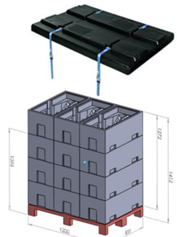
Designed to fit on a standard Euro pallet.
